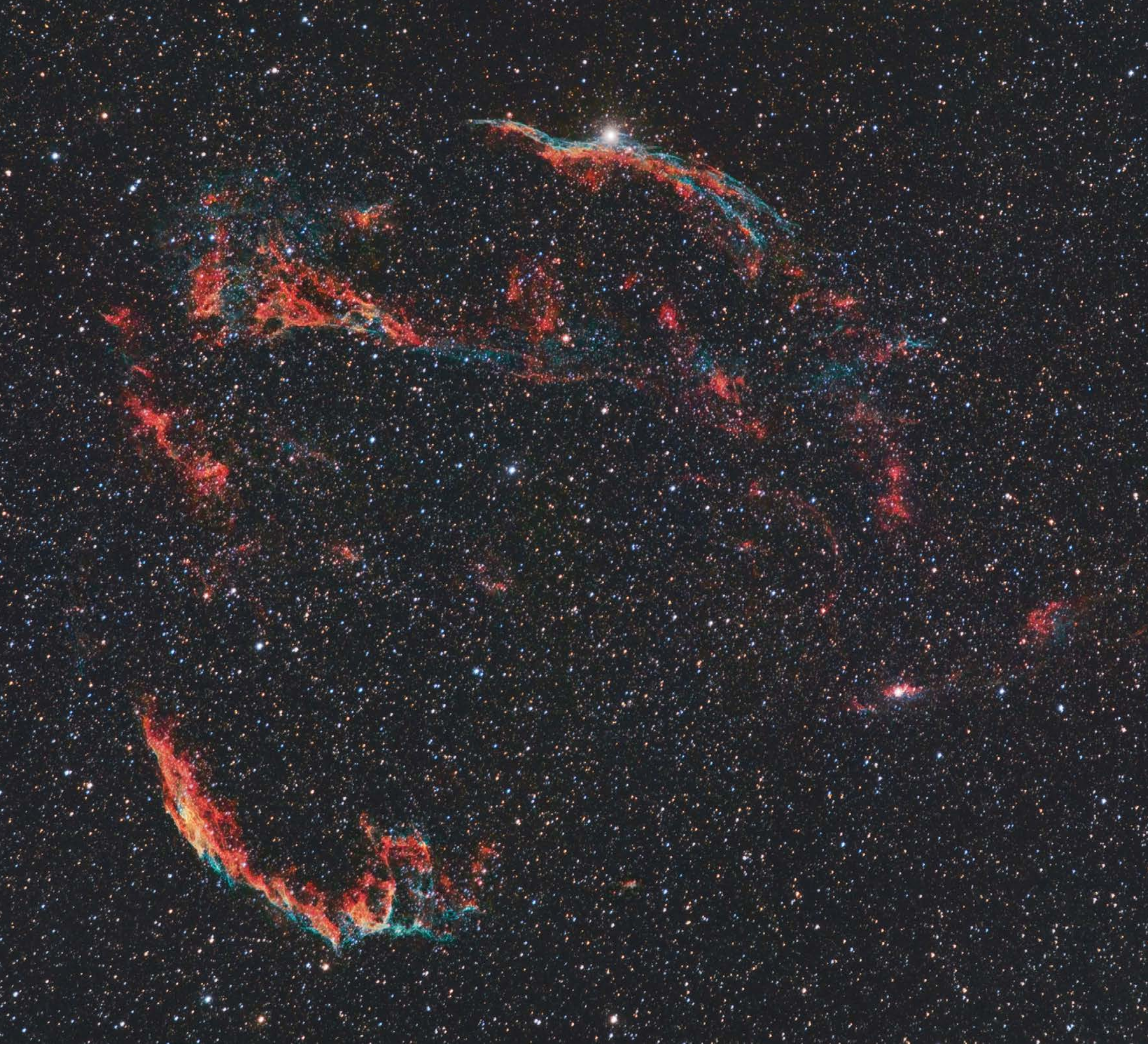
Veil Nebula | Canon 500D modificiran, Canon 70-200 @200 mm f/4, Astronomik CCD CLS filter, ISO 800, 279×80 s (6.2 h) Neven Krčmarek
