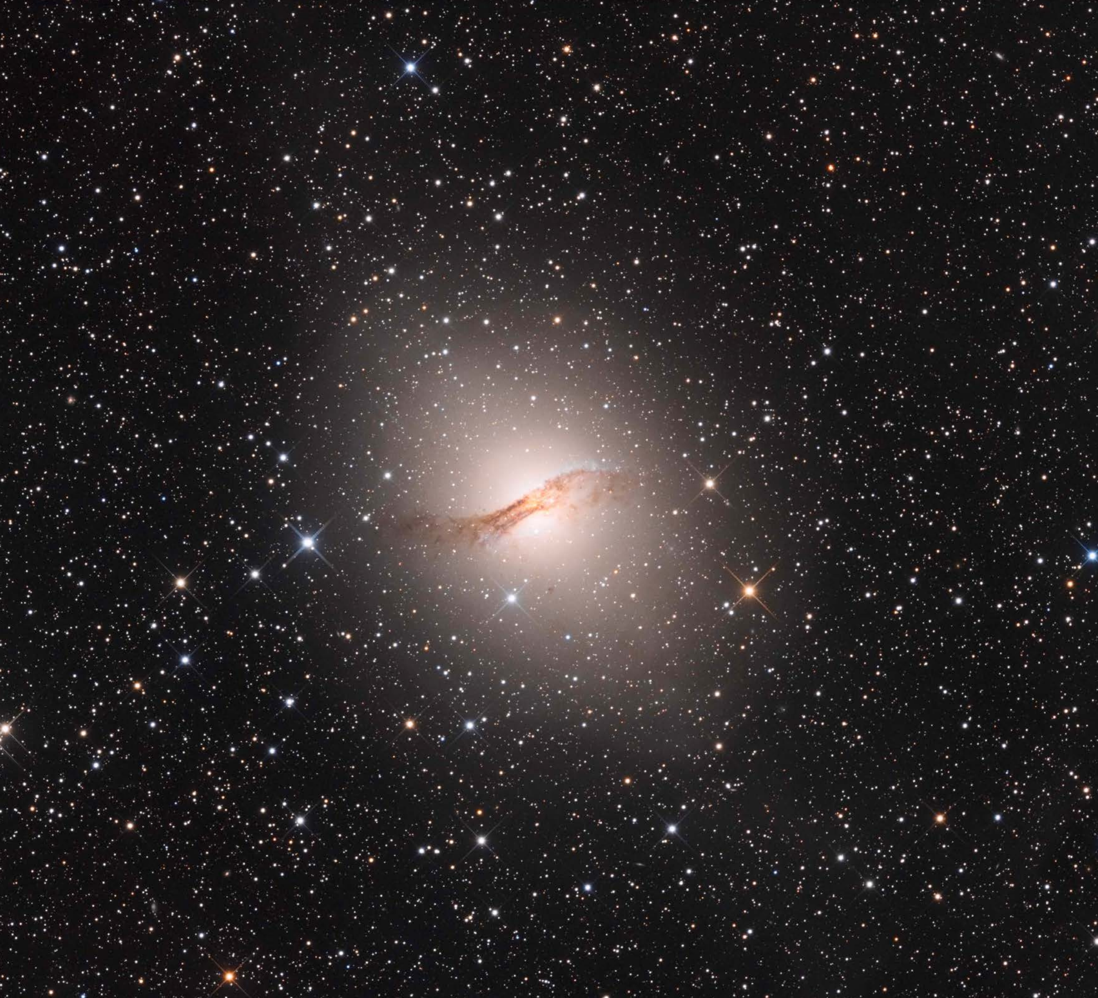
NGC 5128, Centaurus A | Chilescope, 500 mm, f3.6, L 9×300 s, 6×600 s, RGB 6×180 s bin2 (2 h) Veljko Petrović
